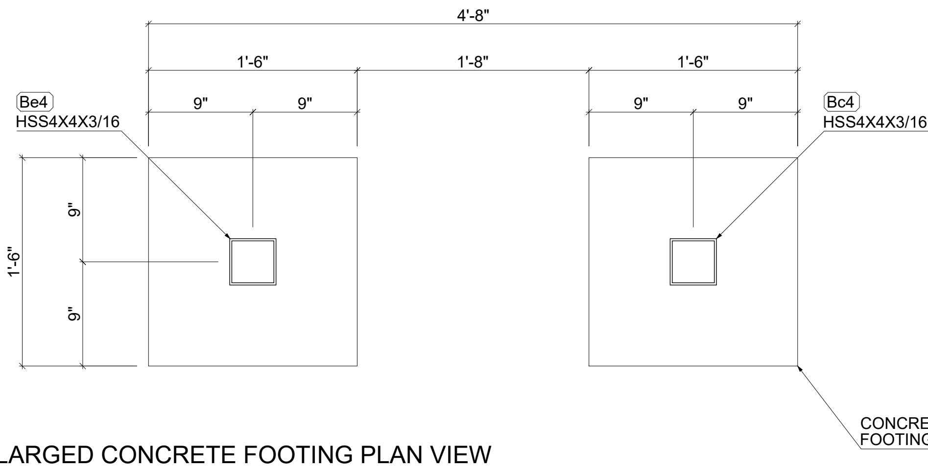
1 ENLARGED CONCRETE FOOTING PLAN VIEW SCALE: 1-1/2" = 1' - 0"
