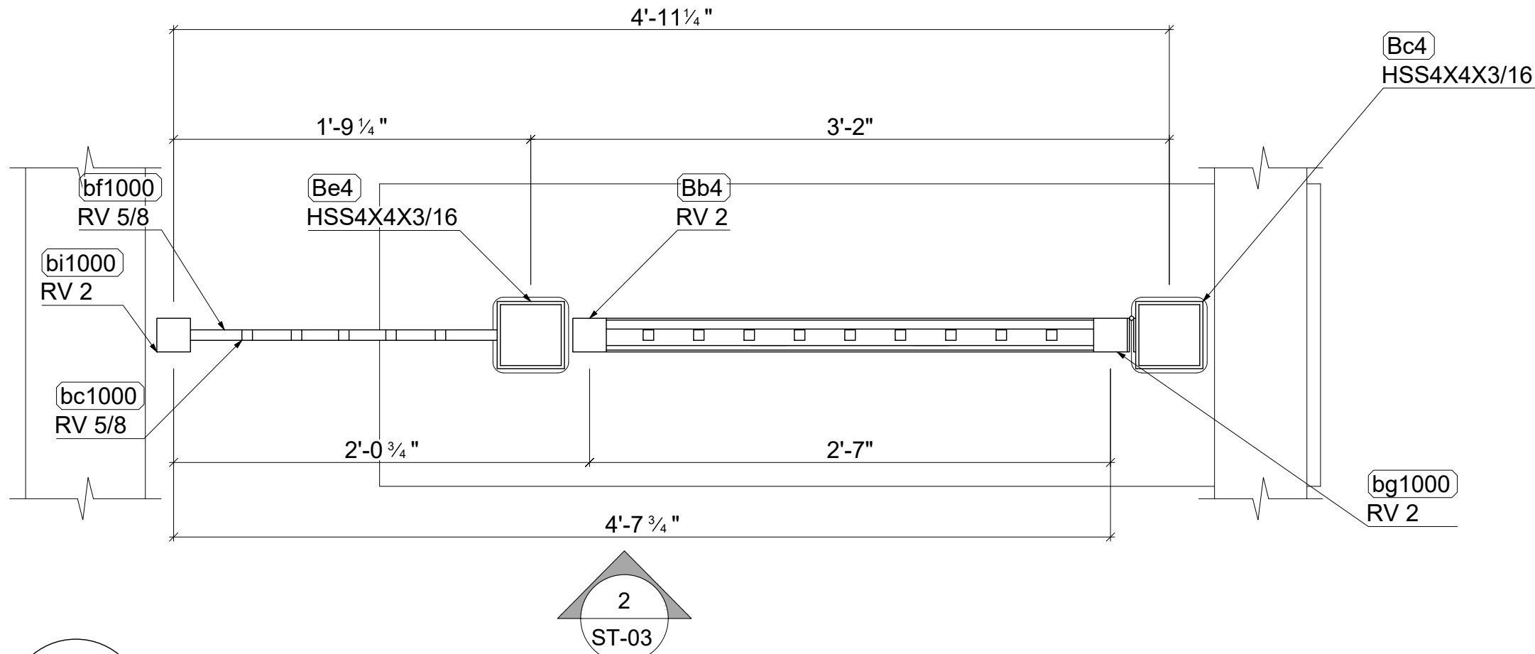
3 ENLARGED GATE PLAN VIEW SCALE: 1-1/2" = 1' - 0"
