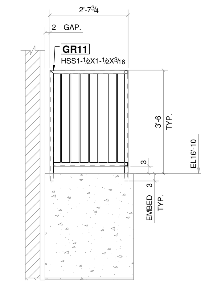
4 STAIR ELEVATION
