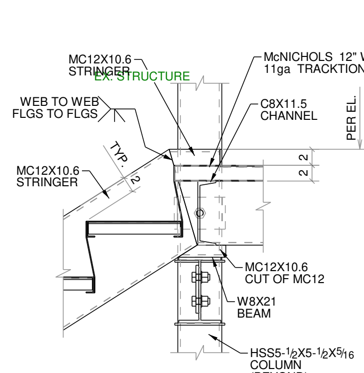
5 DETAIL
