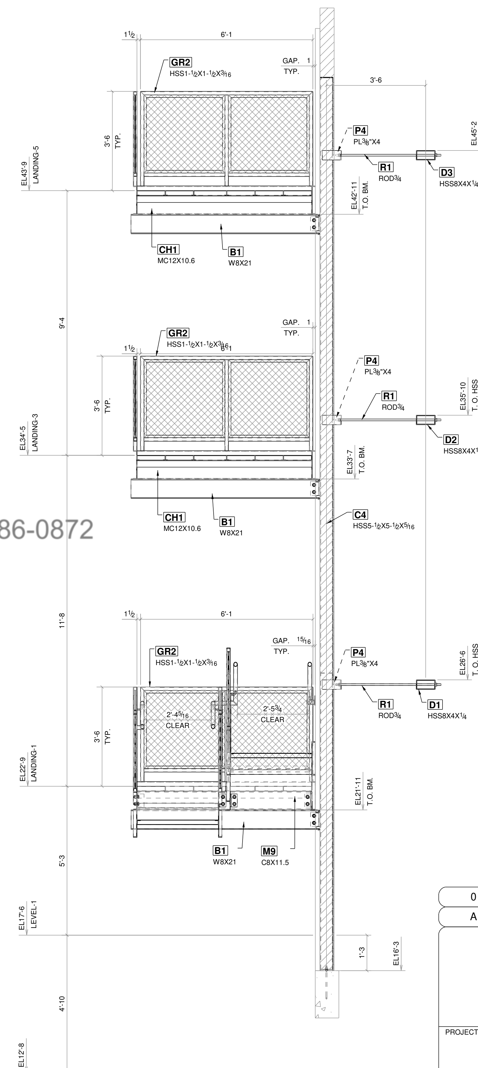
3 STAIR ELEVATION
