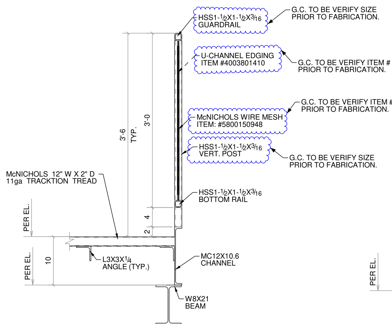
8 TYP. SECTION
