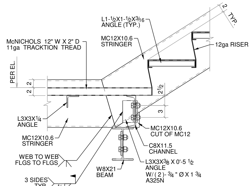
3 DETAIL
