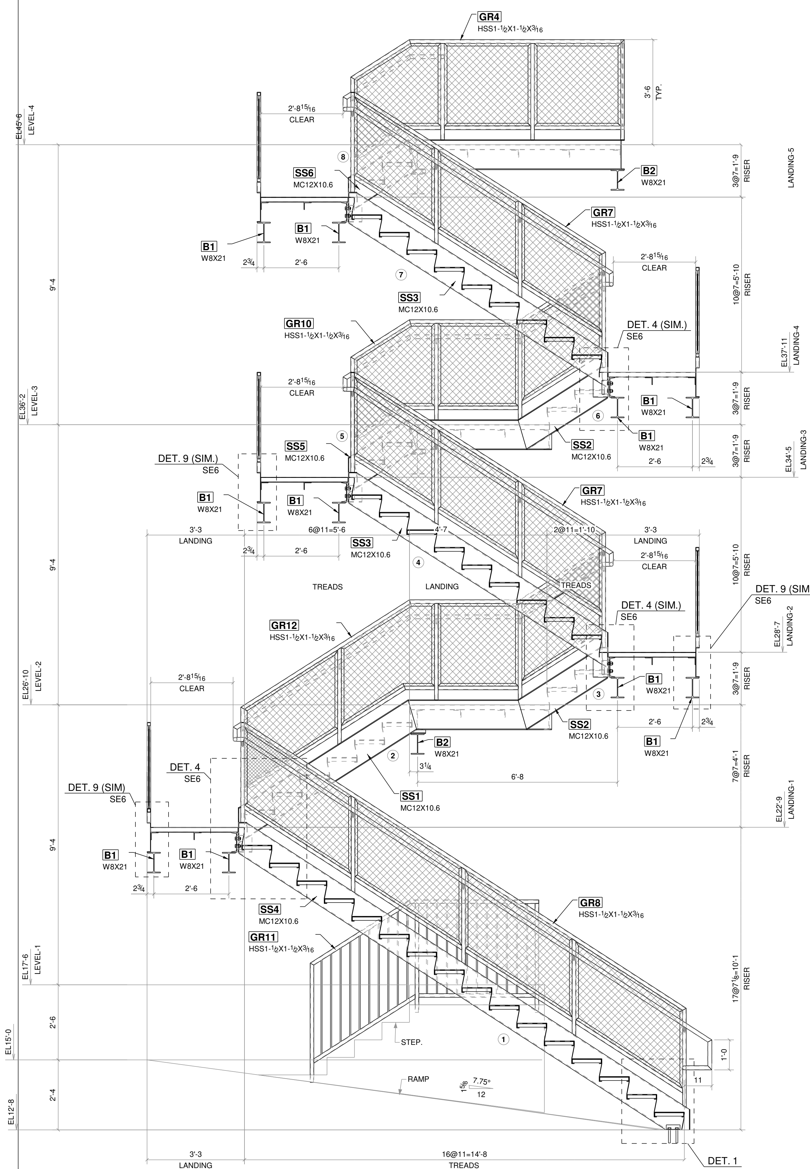
1 STAIR ELEVATION
