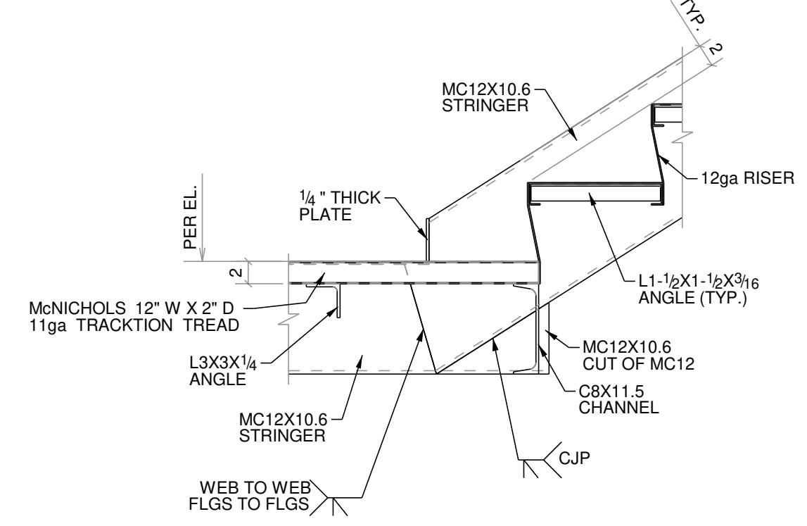
6 DETAIL
