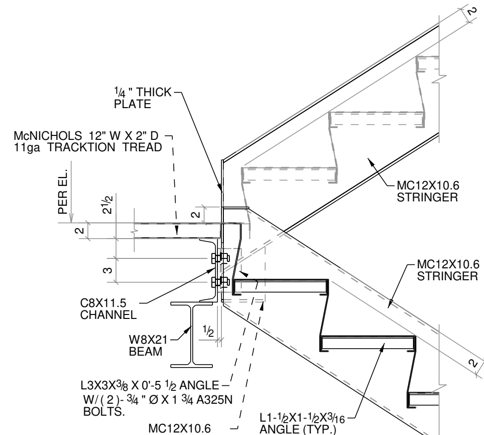
4 DETAIL
