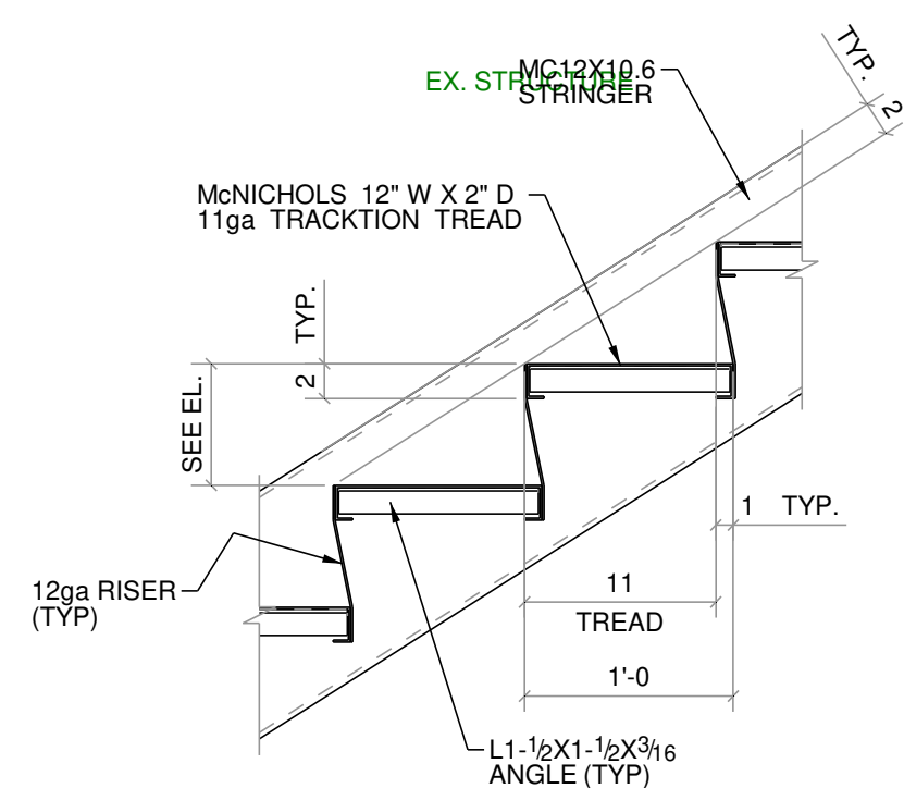
7 DETAIL
