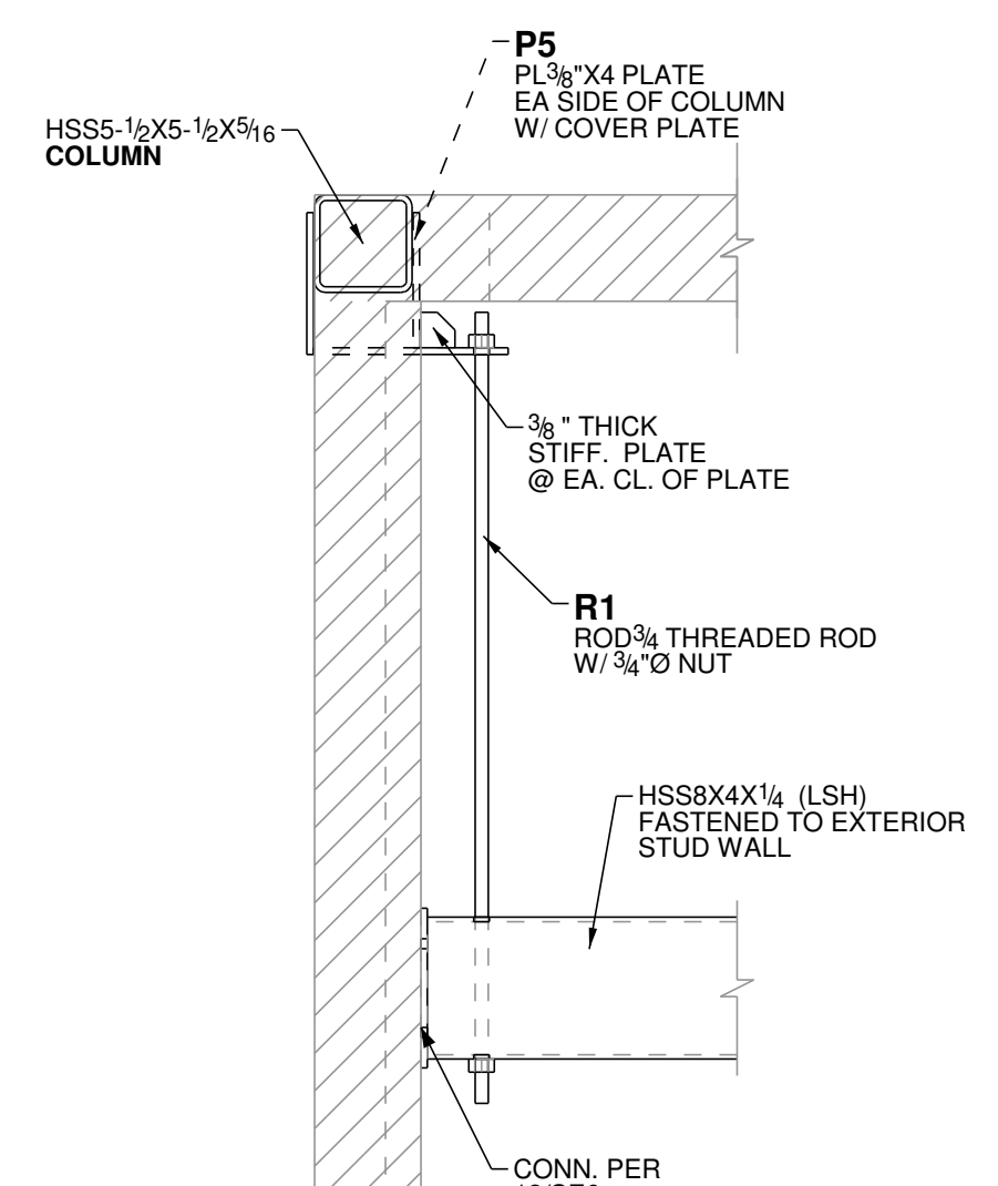
14 TYP. THREADED ROD @ CORNER
