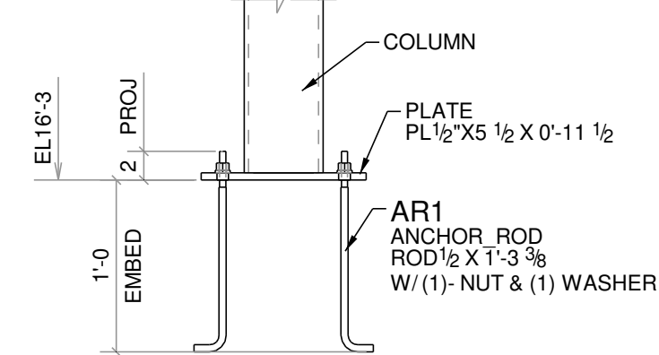
11A ELV. VIEW
