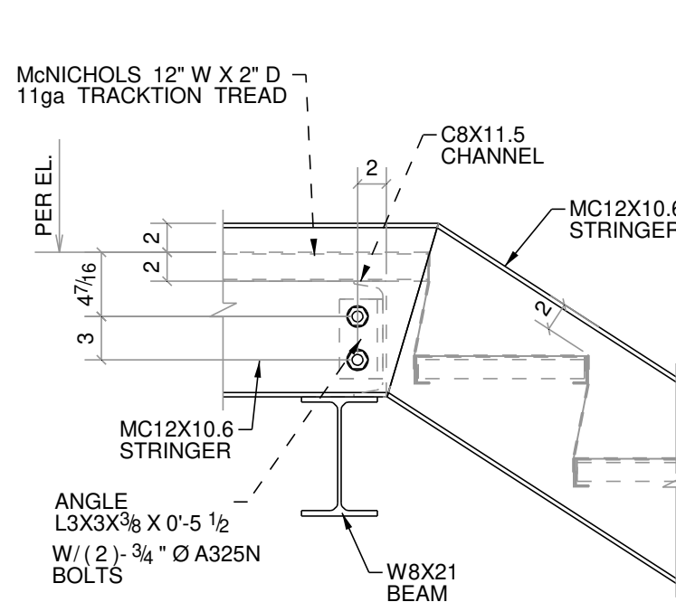
2 DETAIL
