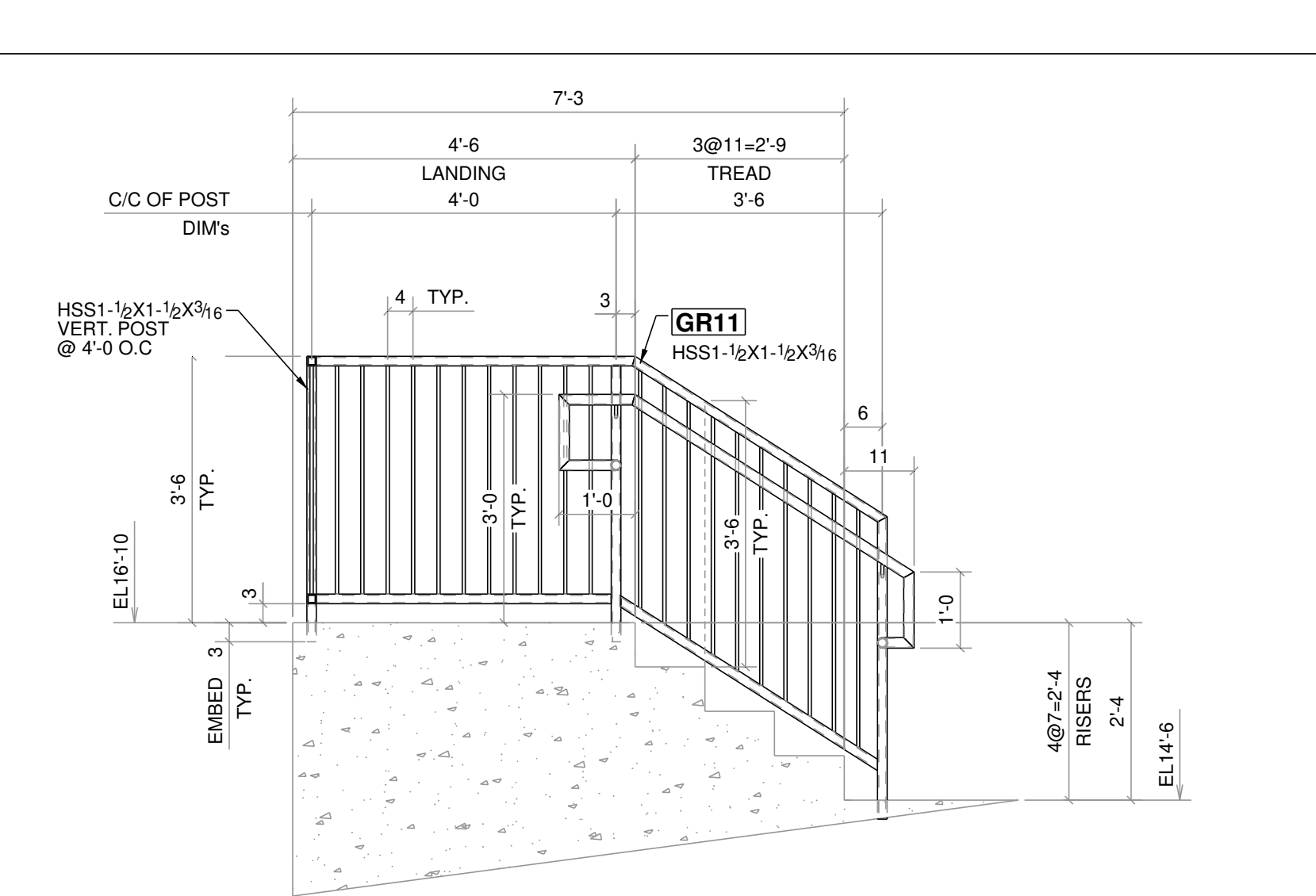
3 STAIR ELEVATION
