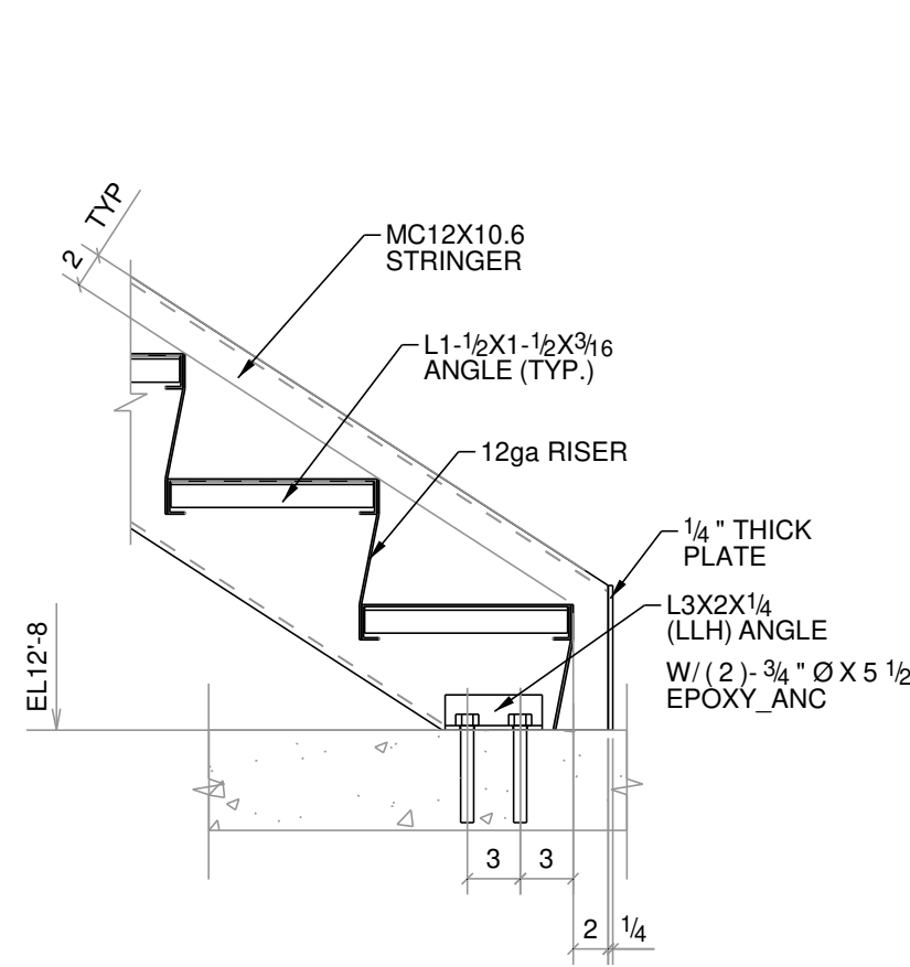
1 TYP. STAIR BASE DETAIL
