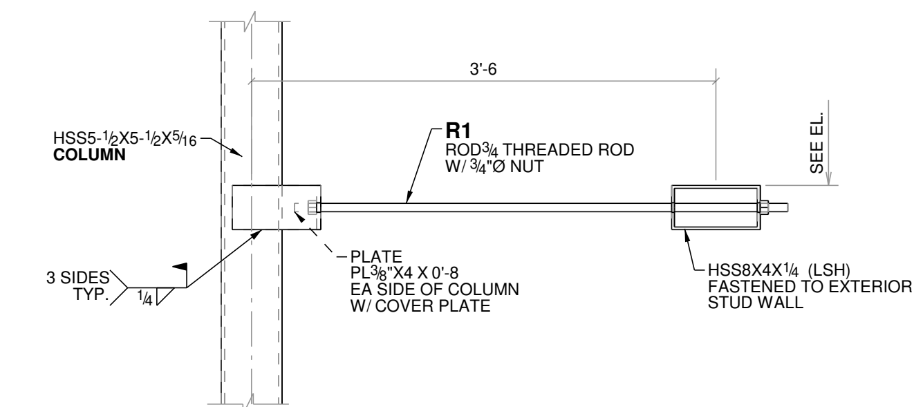
12 TYP. THREADED ROD DETAIL
