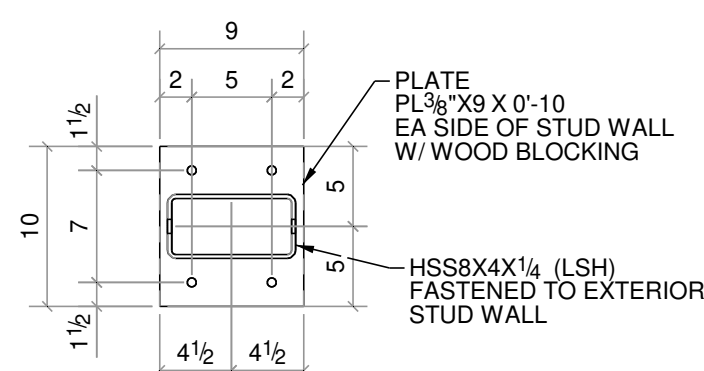
13 DETAIL
