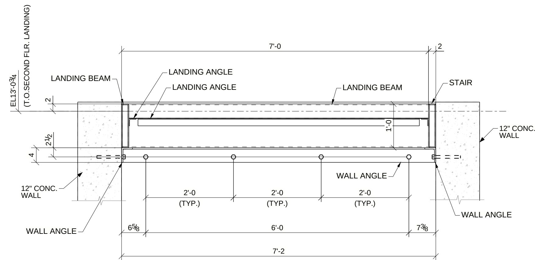
5 LANDING BEAM SECTION @ 2ND FLOOR E8
